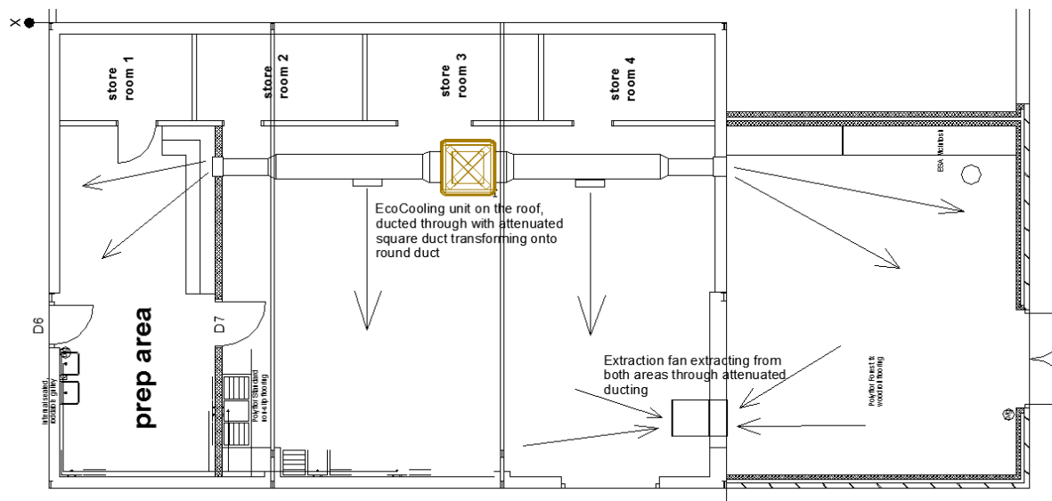
Plan of the area illustrating the EcoCooling unit and attenuated extraction system, one system serves three areas.
